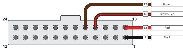
Figure 2. Pin numeration, wire side view
